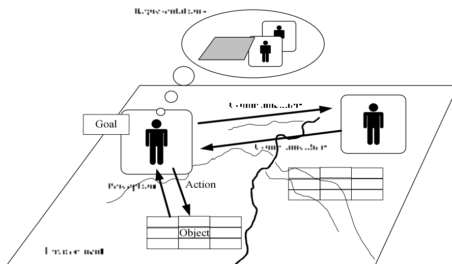
Figure 6.1. Multi-agents system general organization and principles (adapted from Ferber, 1999).
