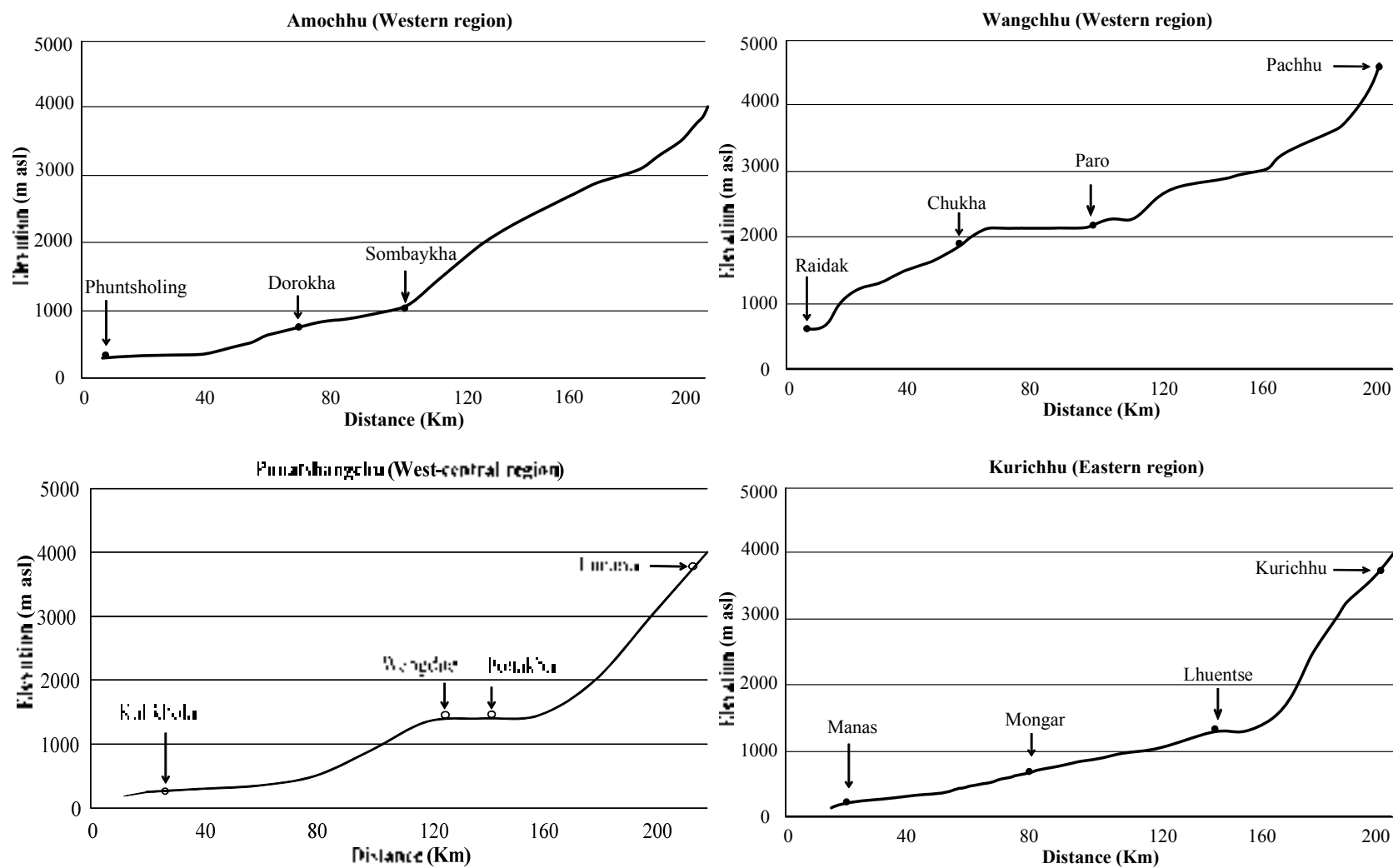
Figure 4.13. Profiles of four major river systems in Bhutan.
