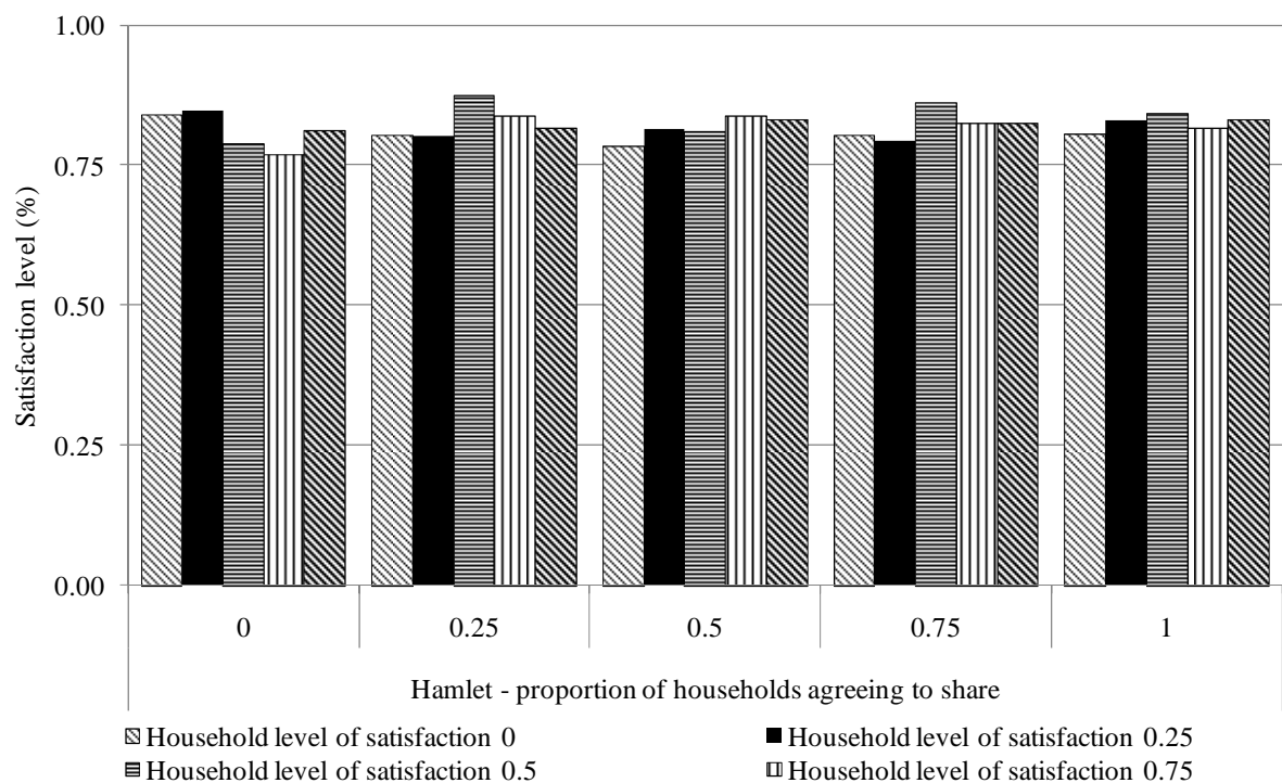
Figure 9.27. Satisfaction level based on sharing rules in different scenario.
