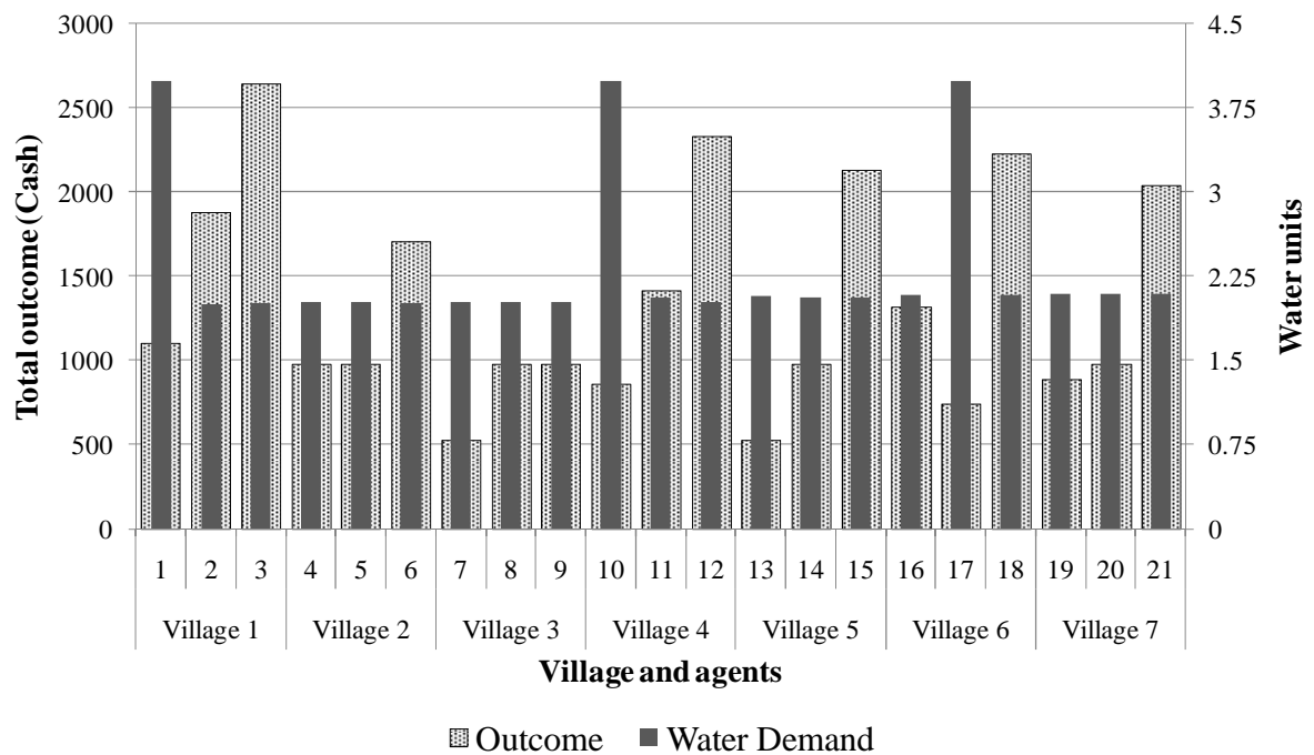
Figure 8.17. Average cash and water demand in open access individual mode simulated with the traditional management regime of the 7 villages agent-based model in Lingmuteychu.
