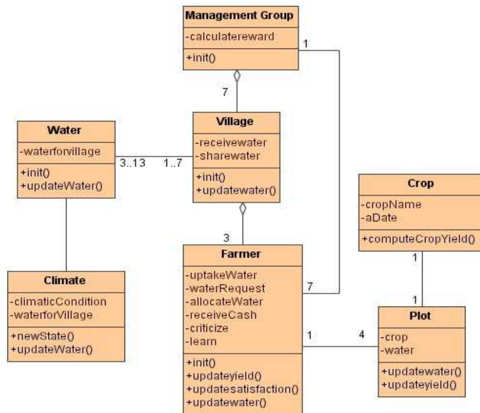
Figure 8.6: UML class diagram showing the attributes and methods associated to each entity in Lingmuteychu 7 villages model.
