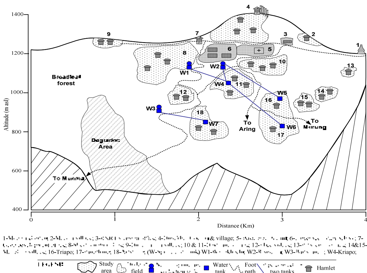
Figure 3.24. Schematic representation of the landscape profile of Kengkhar, Eastern Bhutan.
