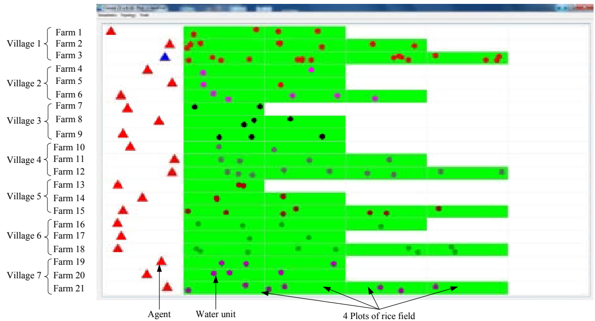
Figure 8.10: CORMAS interface of the seven village agent-based model used in Lingmuteychu.
